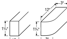
Light Baffle
