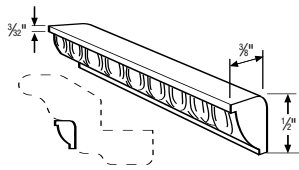
Egg & Dart
