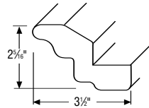
Victorian Crown
