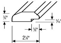
Mirror Frame
