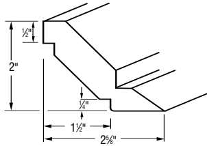
Shaker Crown
