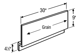
Drop-In Range Front
