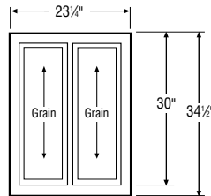
Base Decorative Door Panel Kits
