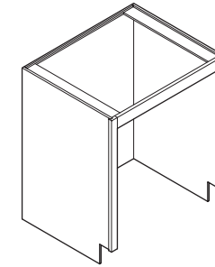
UNIVERSAL DESIGN VANITY SINK BASE 32 1/2" HIGH
