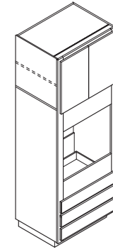
SINGLE OVEN 3 DRAWERS 93" HIGH
